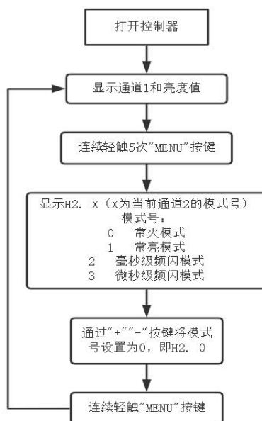
Figure 11 Constant Off Mode Setting Flow Chart
