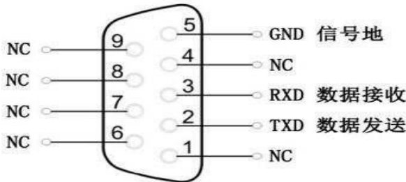
Figure 2 Serial Female Port Interface Definition
