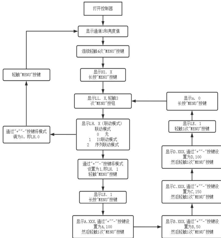
Figure 21 Flow Chart for IO Linkage Mode Setting
