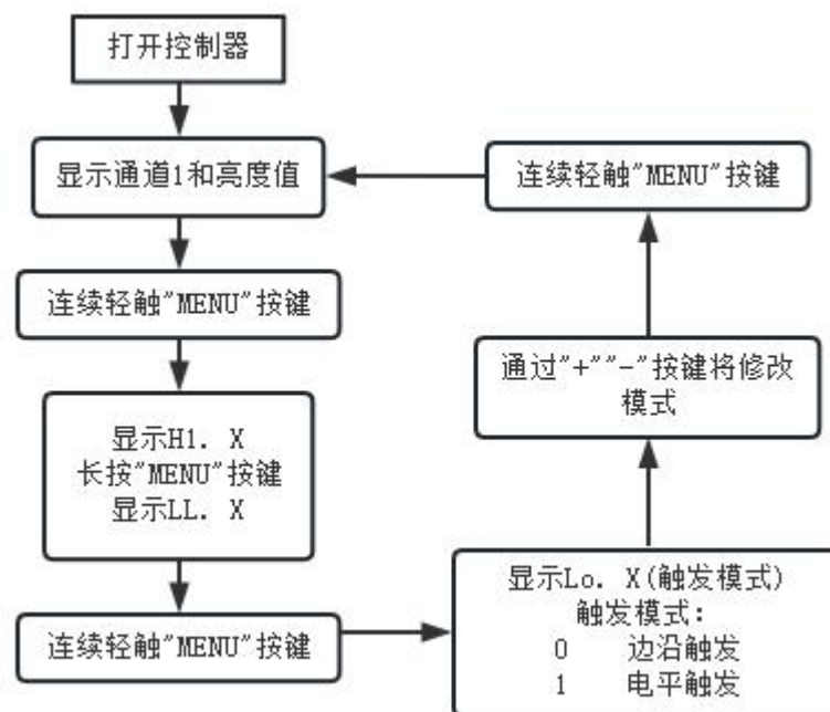
Figure 16 Edge Trigger Mode Setting Flow Chart for All Channels
