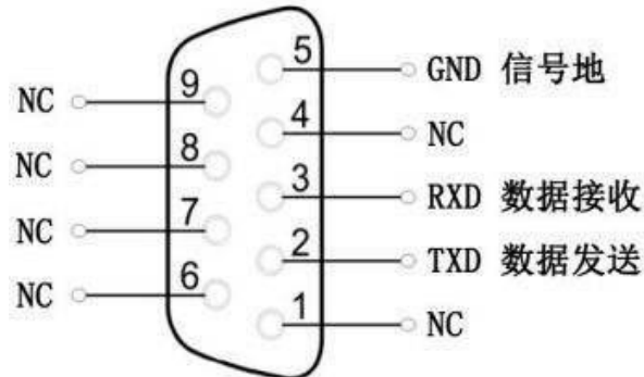
Figure 2: Serial Female Socket Interface Definition
