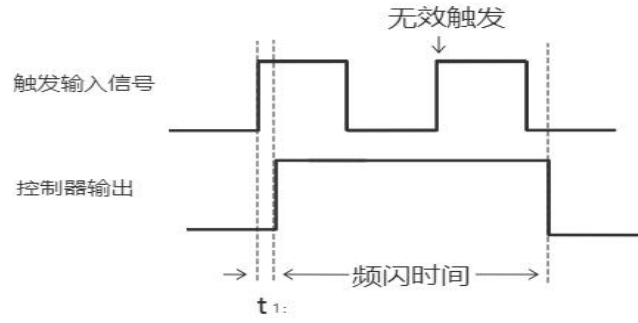
Figure 7: Strobe Mode Timing Diagram
