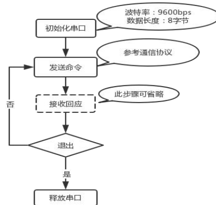
Figure 27: Communication Programming Flow
