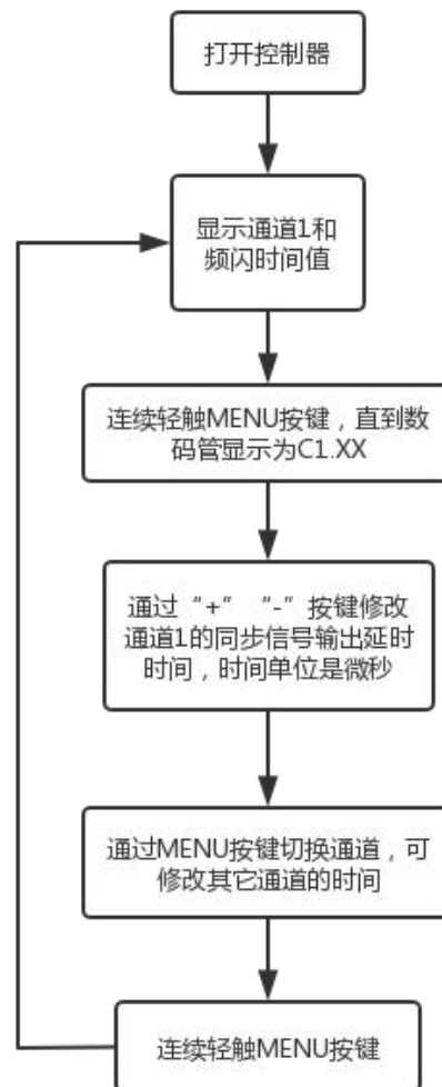
Figure 13: Synchronous Signal Output Delay Setting Flow Chart
