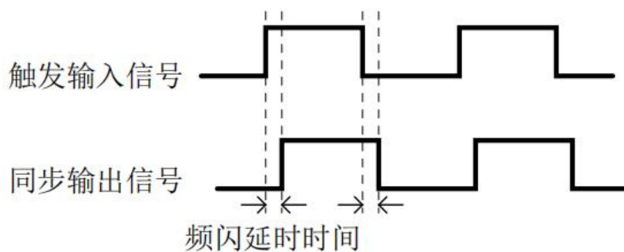
Figure 9: Synchronous Output Signal Timing Diagram
