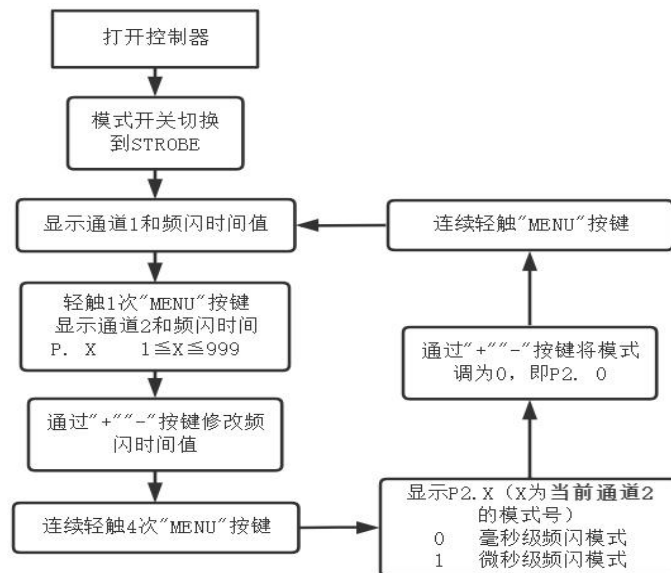
Figure 14 Flow Chart for Millisecond-level Strobe Time Setting
