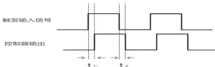
图 Figure 7 Timing Diagram for Constant Off Mode
