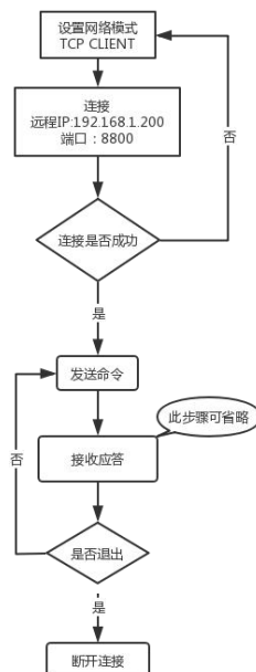
Figure 17 Ethernet Port Communication Programming Flow Chart
