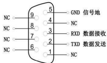
Figure 2 Serial Female Connector Interface Definition
