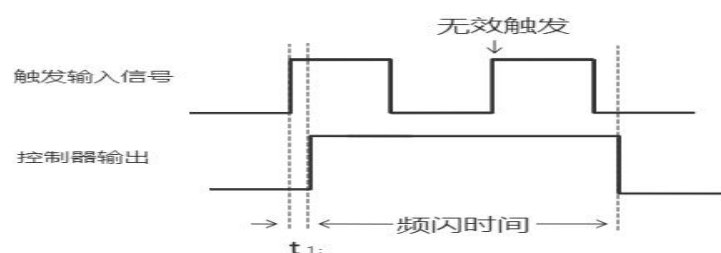
Figure 9 Timing Diagram for Strobe Mode
