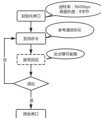
Figure 16 Serial Port Communication Programming Flow Chart
