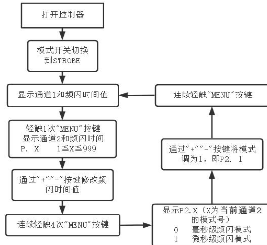
Figure 15 Flow Chart for Microsecond-level Strobe Time Setting
